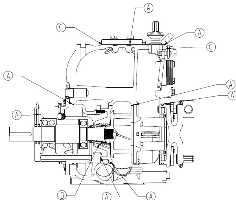
PARTS DRAWING – 372000153 MECHANICAL SEAL PARTS KITS
