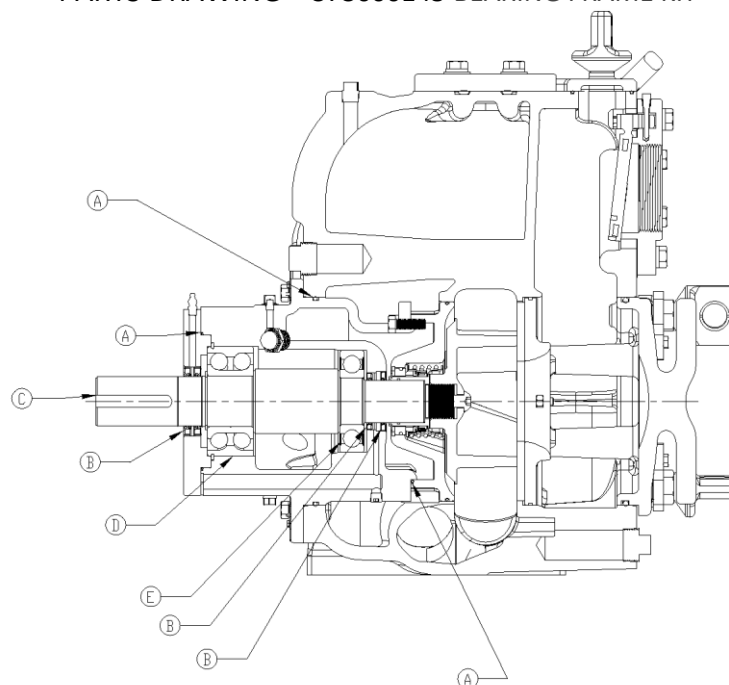
PARTS DRAWING – 373000145 BEARING FRAME KIT
