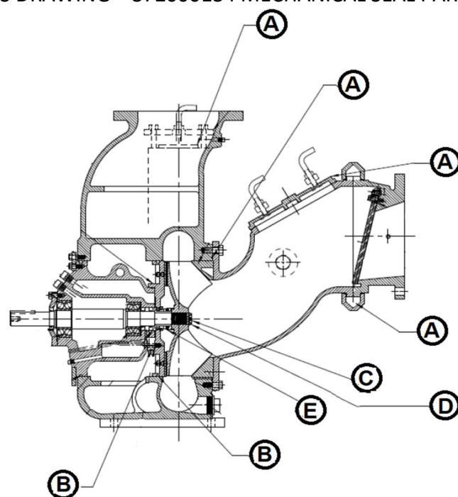
PARTS DRAWING – 372000134 MECHANICAL SEAL PARTS KITS
