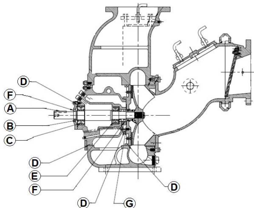
PARTS DRAWING – 373000130 BEARING FRAME KIT
