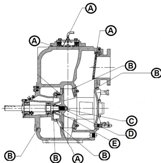
PARTS DRAWING – 372000135 MECHANICAL SEAL PARTS KITS
