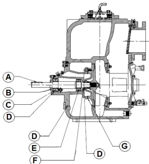
PARTS DRAWING – 373000131 BEARING FRAME KIT
