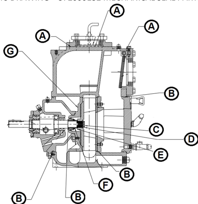
PARTS DRAWING – 372000132 MECHANICAL SEAL PARTS KITS
