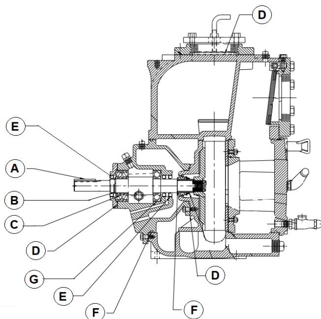
PARTS DRAWING – 373000128 BEARING FRAME KIT
