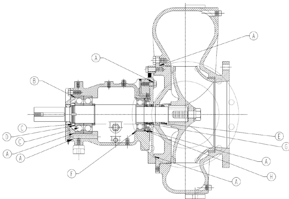
PARTS DRAWING – 373000135 BEARING FRAME PARTS KIT
