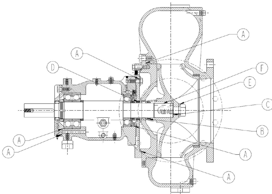
PARTS DRAWING – 372000149 MECHANICAL SEAL PARTS KIT
