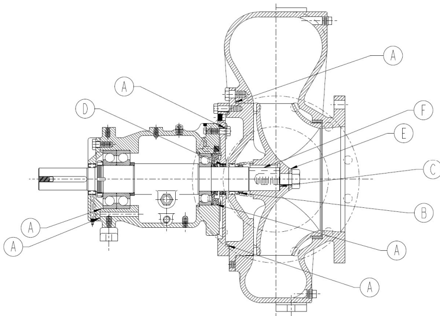
PARTS DRAWING – 372000149 MECHANICAL SEAL PARTS KITS
