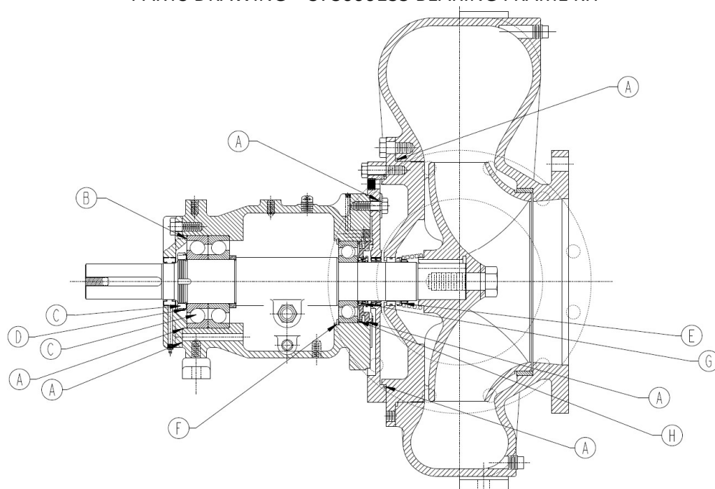
PARTS DRAWING – 373000135 BEARING FRAME KIT
