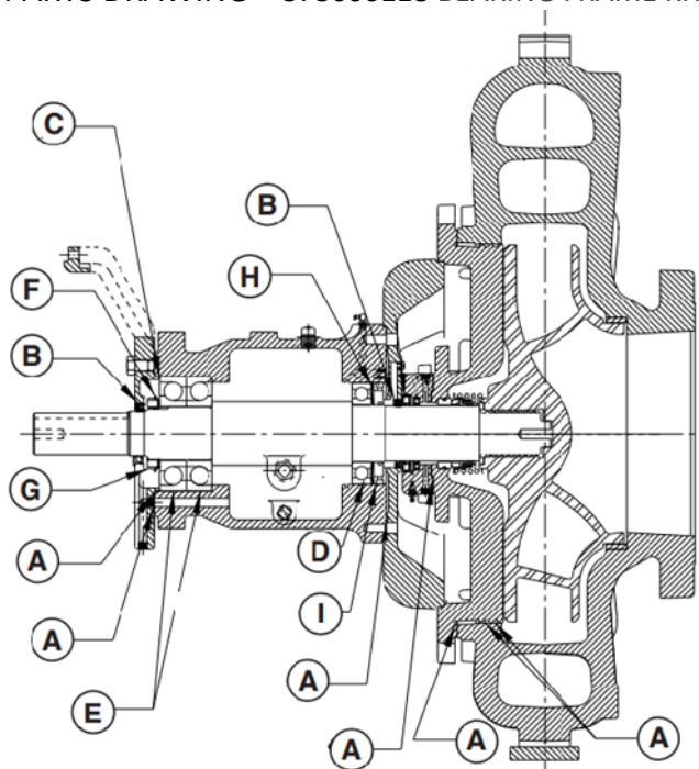
PARTS DRAWING – 373000118 BEARING FRAME KIT
