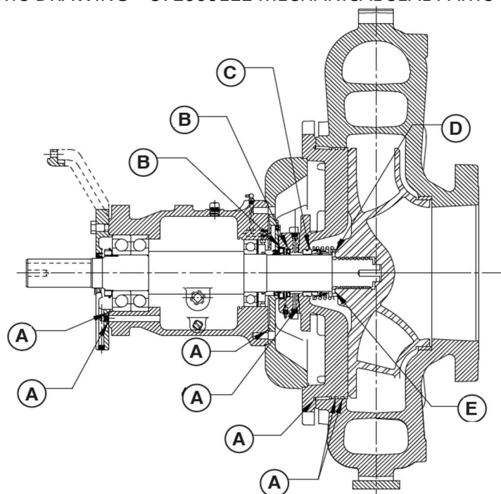
PARTS DRAWING – 372000122 MECHANICAL SEAL PARTS KITS
