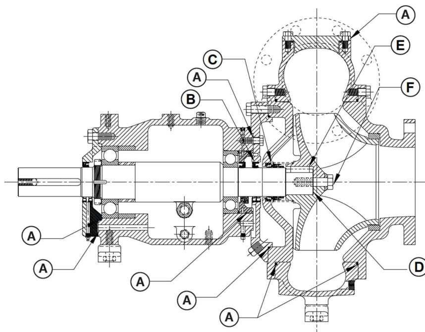
PARTS DRAWING – 372000101 MECHANICAL SEAL PARTS KITS
