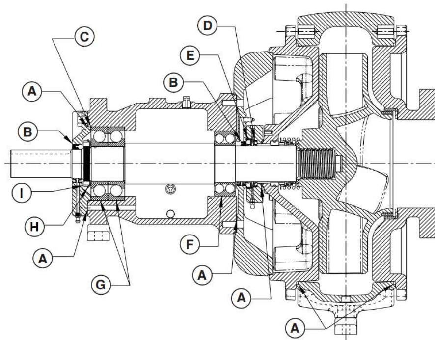
PARTS DRAWING – 373000120 BEARING FRAME KIT
