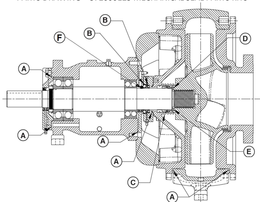
PARTS DRAWING – 372000125 MECHANICAL SEAL PARTS KITS
