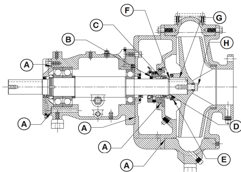
PARTS DRAWING – 372000111 MECHANICAL SEAL PARTS KITS
