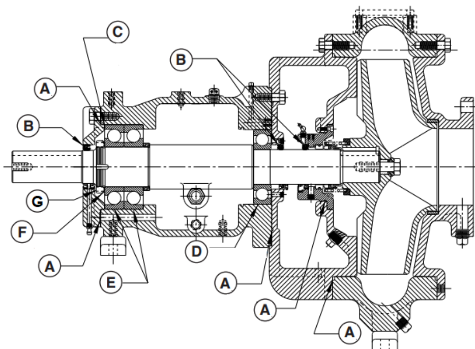
PARTS DRAWING – 373000112 BEARING FRAME KIT
