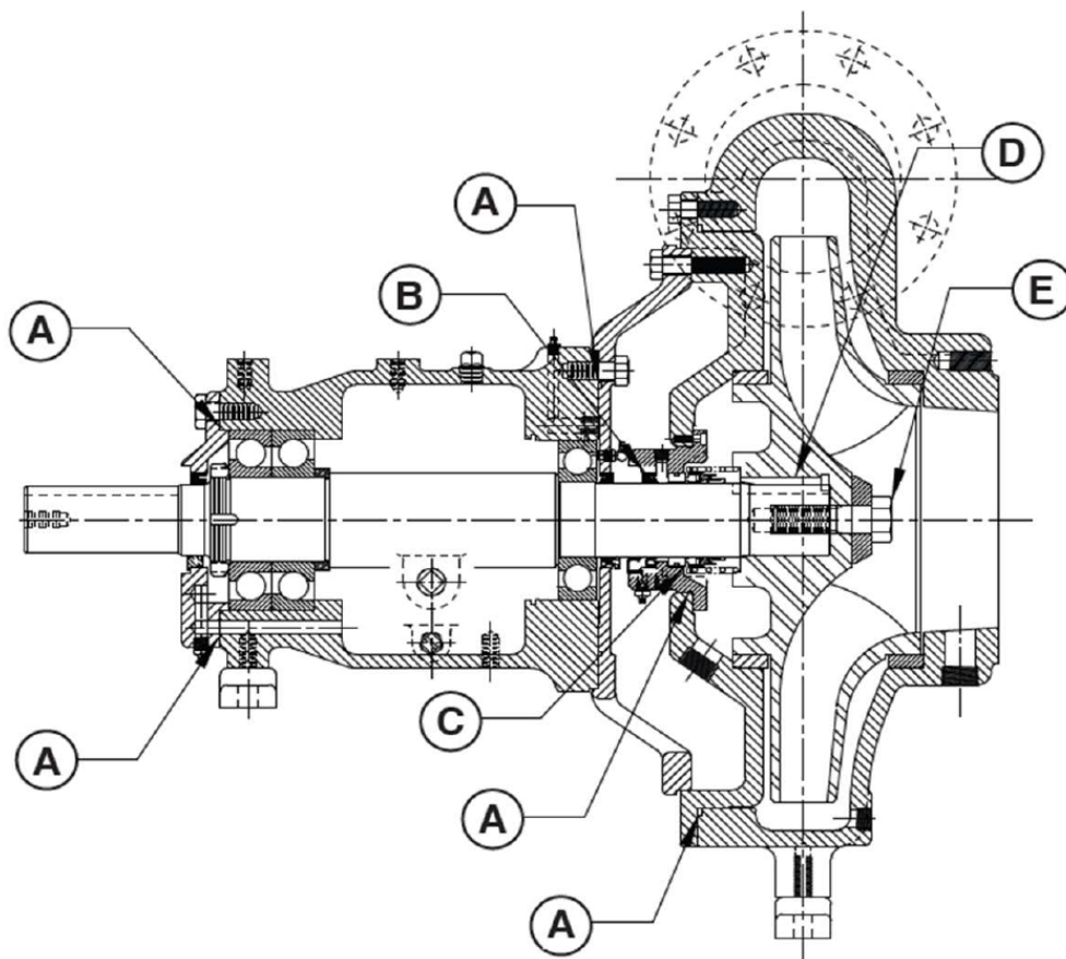
PARTS DRAWING – 372000119 MECHANICAL SEAL PARTS KIT
