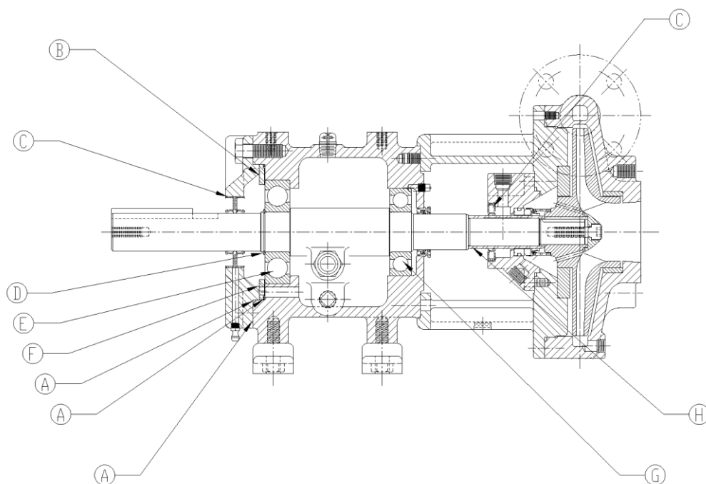
PARTS DRAWING – 373000143 BEARING FRAME KIT
