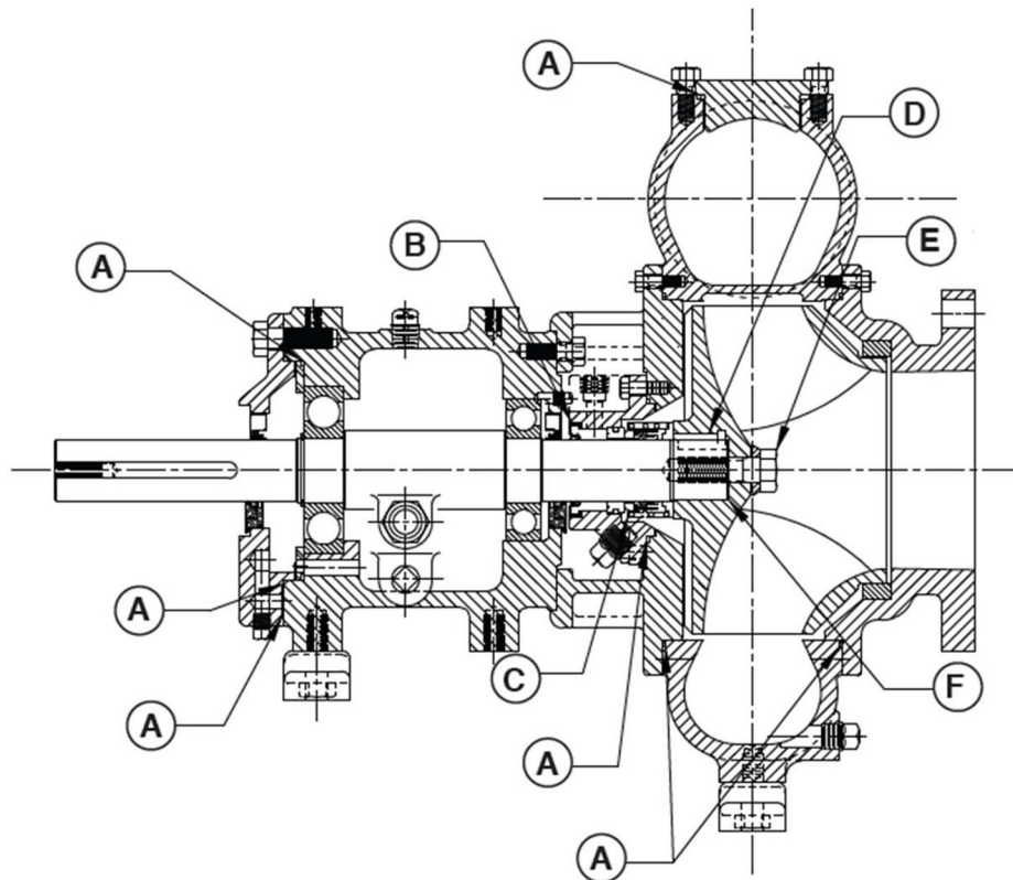
PARTS DRAWING – 372000105 MECHANICAL SEAL PARTS KIT
