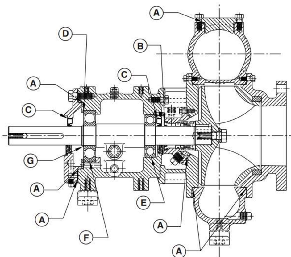
PARTS DRAWING – 373000109 BEARING FRAME PARTS KIT
