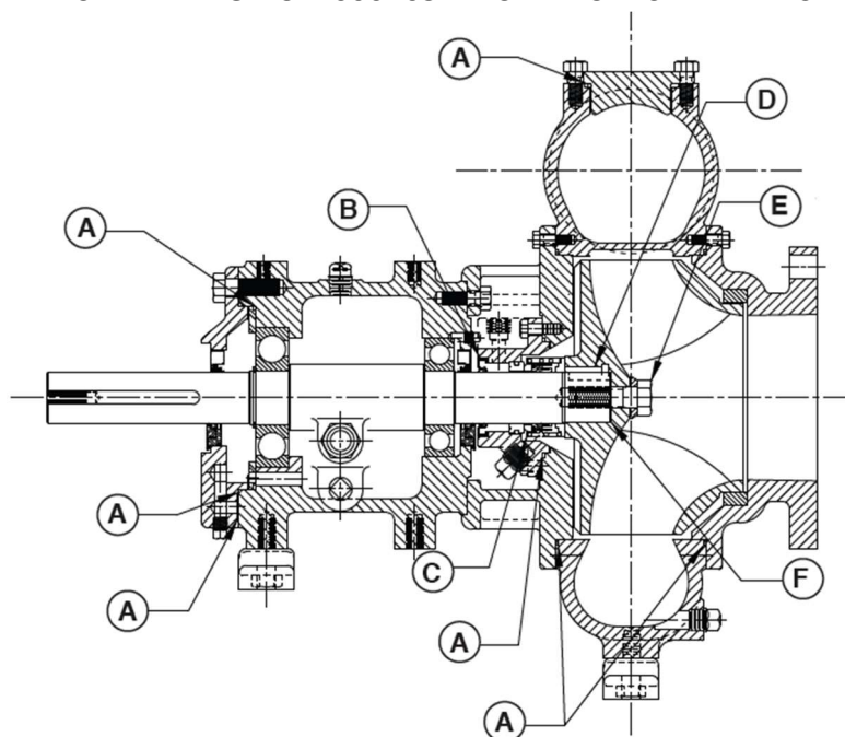
PARTS DRAWING – 372000105 MECHANICAL SEAL PARTS KITS
