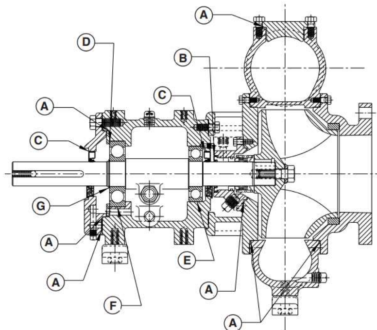
PARTS DRAWING – 373000109 BEARING FRAME KIT
