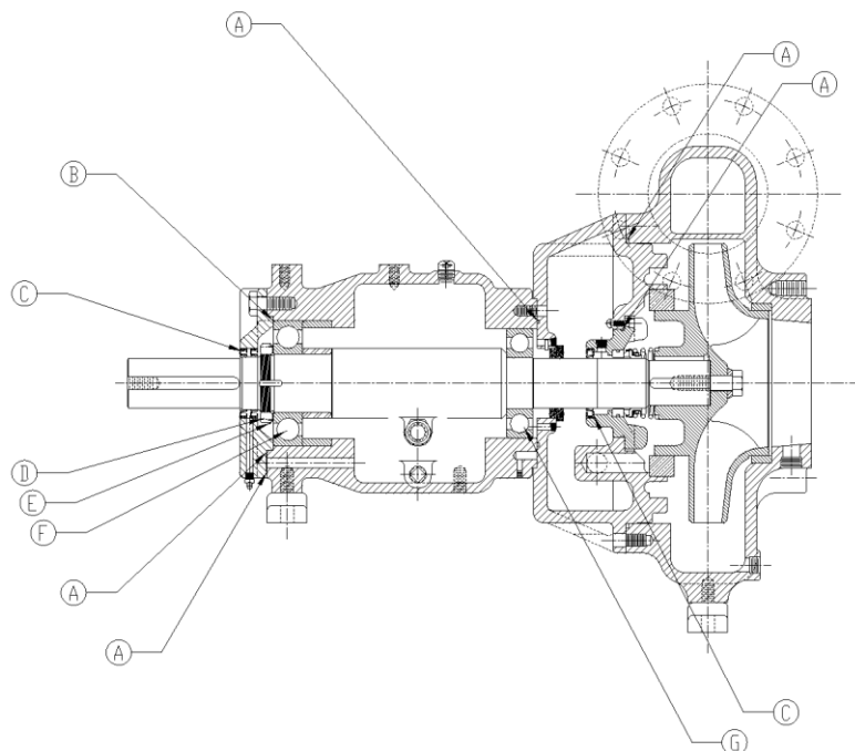
PARTS DRAWING – 373000147 BEARING FRAME KIT
