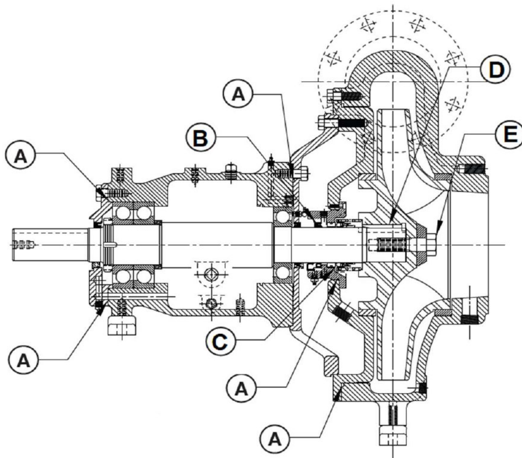
PARTS DRAWING – 372000120 MECHANICAL SEAL PARTS KIT
