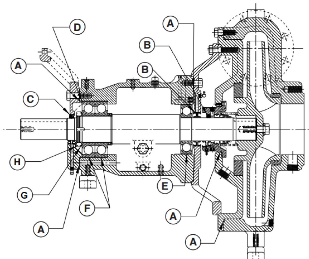
PARTS DRAWING – 373000117 BEARING FRAME PARTS KIT
