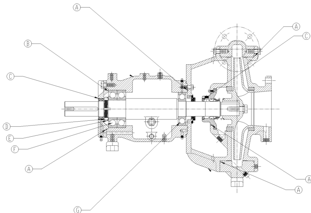
PARTS DRAWING – 373000108 BEARING FRAME KIT
