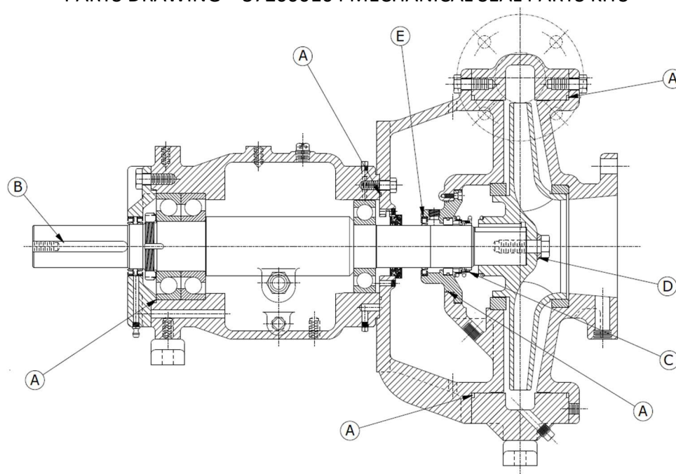
PARTS DRAWING – 372000104 MECHANICAL SEAL PARTS KITS
