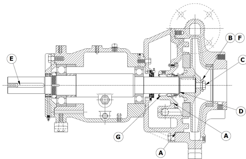
PARTS DRAWING – 372000117 MECHANICAL SEAL PARTS KITS
