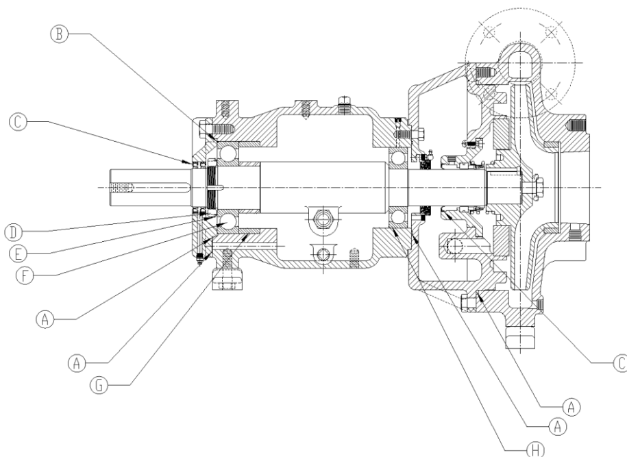
PARTS DRAWING – 373000115 BEARING FRAME KIT
